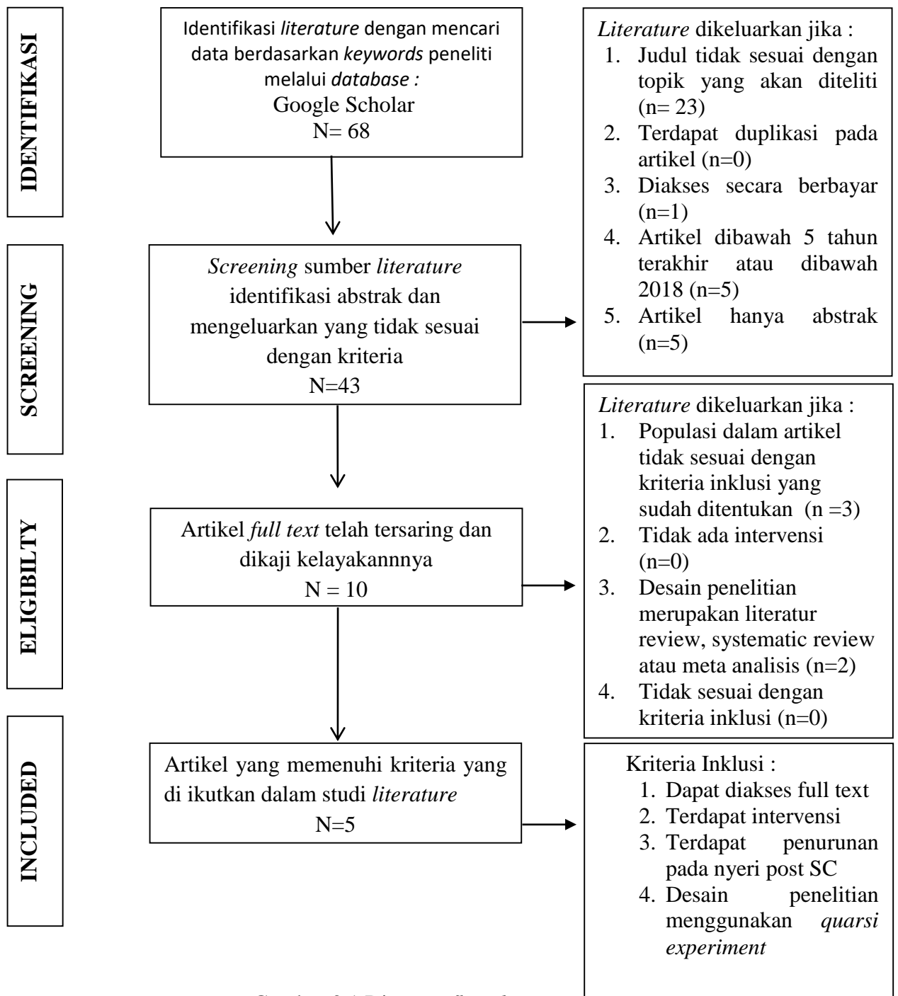
Gambar 3.1 Diagram flowchart
